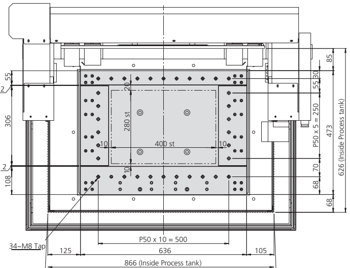
Work Table
